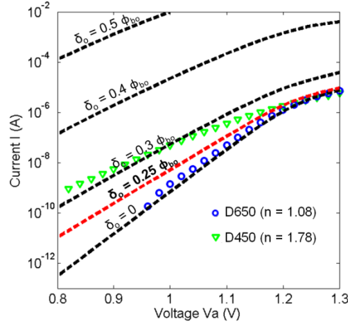
Figure 4.10 Diode current at various \delta_o/\phi_{\text{bulk}} ratios. D450 and D650 are placed alongside for reference. The curve denoted by \delta_o = 0 curve shows the ideal thermionic emission characteristics ( n = 1 ).
