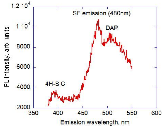
Figure 3.21 Emission line at 480nm from a 20um thick epilayer with IGFS density >10,000 \text{ cm}^{-2} at an excitation wavelength of 310nm.
