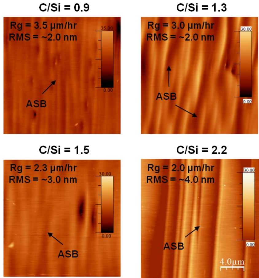
Figure 3.15 AFM images ( 20\mu\text{m} \times 20\mu\text{m} ) of 1^\circ offcut epilayers grown at various C/Si ratios. The arrows show regions with anisotropic step bunching. The growth duration was 1 hour for all of the epilayers.
